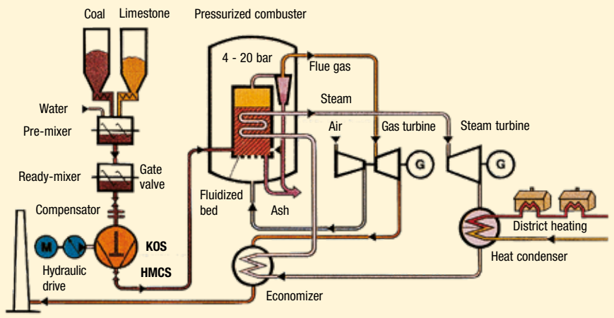
Coal injection with pressurized fluidized-bed combustor. The flow chart shows a combined gas and steam turbine process with pressurized fluidized-bed combustion. (ABB Carbon)
